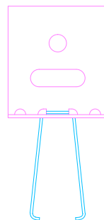
34.4425 SUSPENSION BRACKET WITH CLAMP-front
