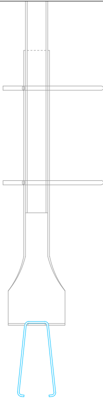
CLIP-IN LOWER NONIUS HANGER COMPLETE-front
