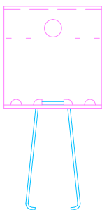
34.4410 CROSS CONNECTOR WITH CLAMP-front
