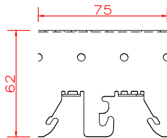
CARRIER 300AC-side
