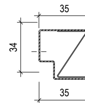
EDGE-PROFILE UW 30 L= max.3000 mm
