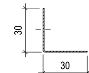
EDGE-PROFILE L 30 L= max.3000 mm
