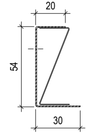
EDGE-PROFILE U 50 L= max.3000 mm
