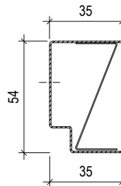
EDGE-PROFILE UW 50 L= max.3000 mm
