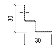
EDGE-PROFILE W 30 L= max.3000 mm
