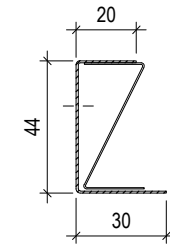
EDGE-PROFILE U 40 L= max.3000 mm
