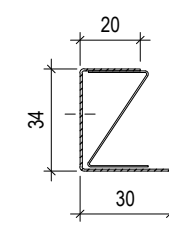
EDGE-PROFILE U 30 L= max.3000 mm
