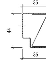
EDGE-PROFILE UW 40 L= max.3000 mm
