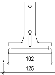
Front view 125
