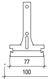
Front view 100
