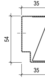
EDGE-PROFILE UW 50 L= max.3000 mm
