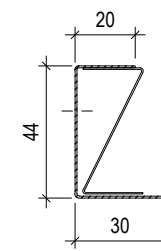
EDGE-PROFILE U 40 L= max.3000 mm
