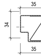
EDGE-PROFILE UW 30 L= max.3000 mm
