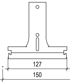
Front view 150
