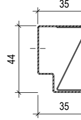
EDGE-PROFILE UW 40 L= max.3000 mm
