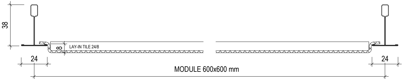
T-PROFILE 38x24 (non HD) side
