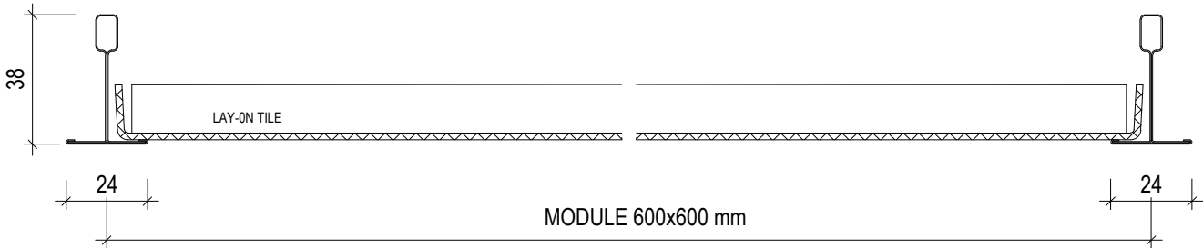
T-PROFILE 38x24 (non HD) side
